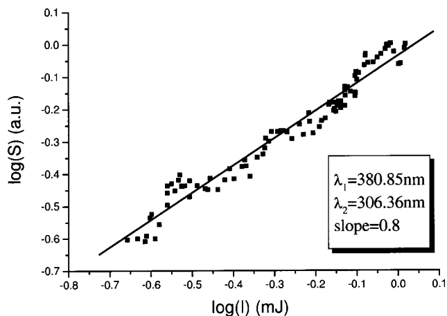
FIG. 3. Dependence of \text{SO}^+ ion signal on laser intensity in double logarithmic form obtained with \lambda_1=380.85 nm and \lambda_2=306.36 nm for ionization laser and dissociation laser, respectively. The slope of regression line is 0.8.
